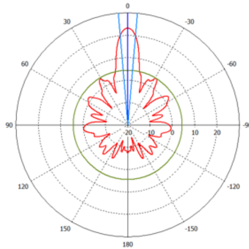
Radiation pattern Vertical Plane
